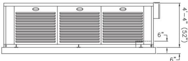
ELEVATION (FRONT VIEW)
