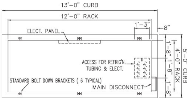
PLAN VIEW (FRONT VIEW)
