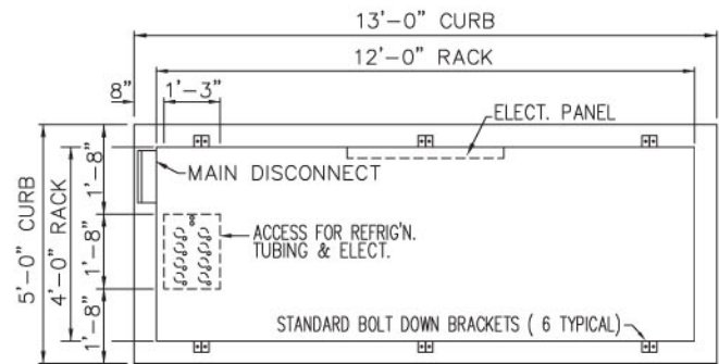
PLAN VIEW (REAR VIEW)
