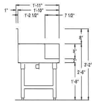
"S" SECTION (Less Sink)
