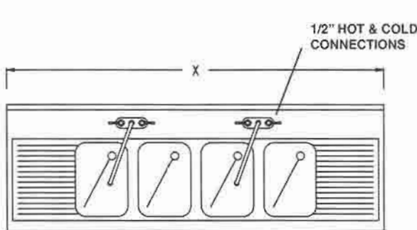
"D" PLAN
