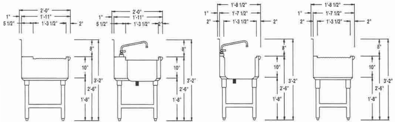
"D" SECTIONS
