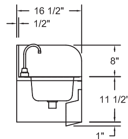
SECTION
